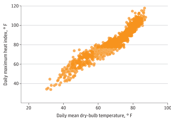
Figure 2. Estimated Maximum Daily Heat Index for Total Sample, 2015 to 2017
